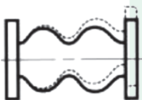
Horizontal Displacement
